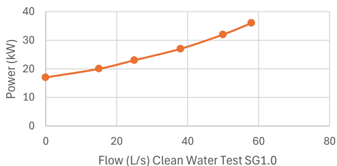
Power Curve 125mm Titan-37Kw 4P
