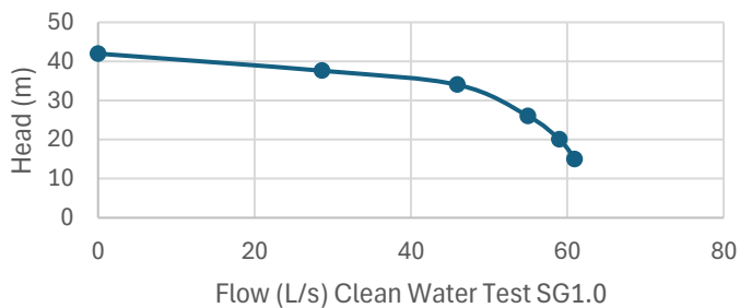
Pump Curve 125mm Titan-37kw 4P STD
