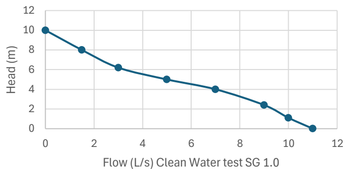
Pump Curve 40mm Titan - 5.5kw 4P
