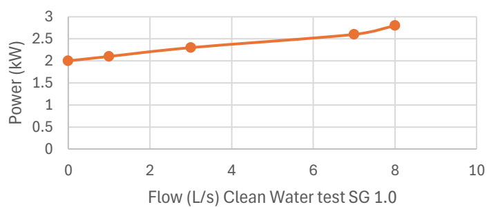
Power Curve 40mm Titan - 5.5kw 4P
