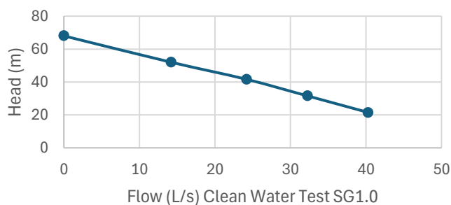
Pump Curve 65mm Titan - 37kw 2P
