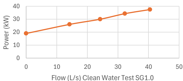
Power Curve 65mm Titan - 37kw 2P
